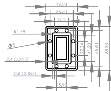
FLANGE DETAIL
